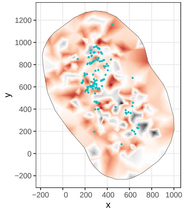
Post. sample
