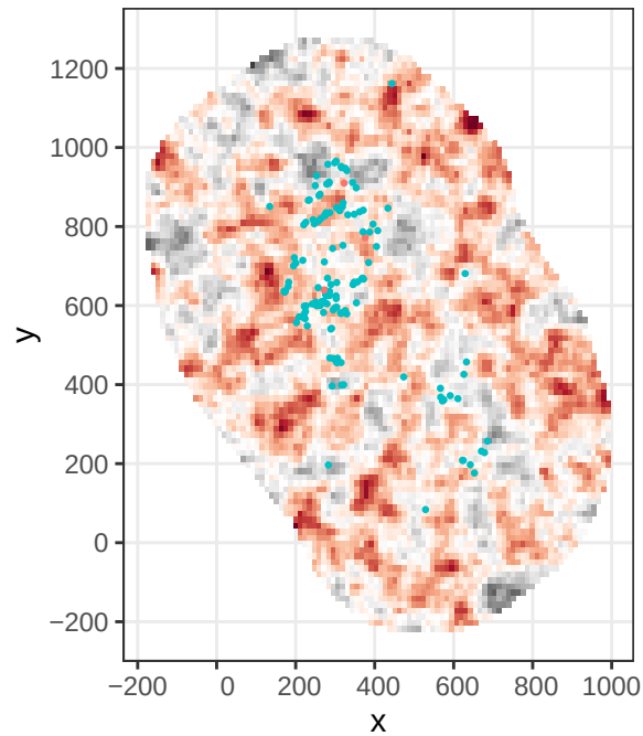
True field
