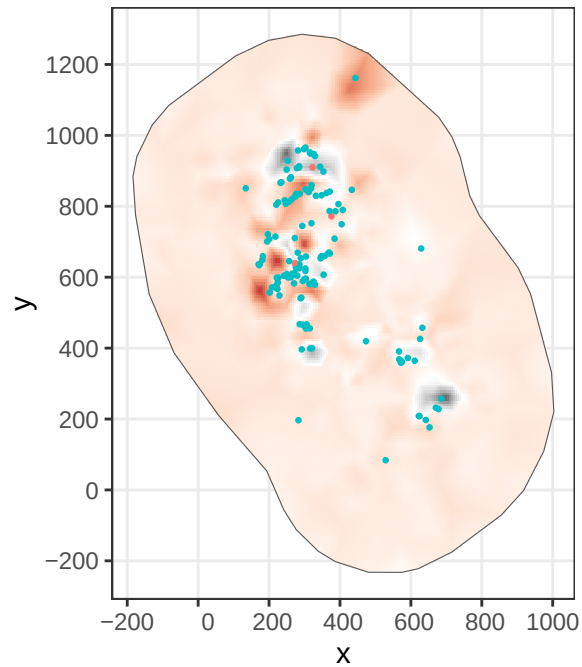
Post. mean
