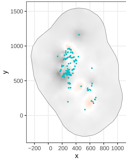
Post. mean
