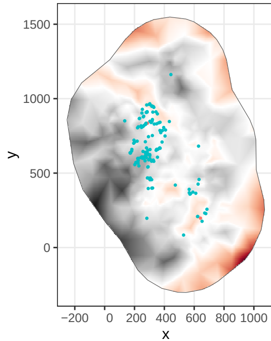
Post. sample
