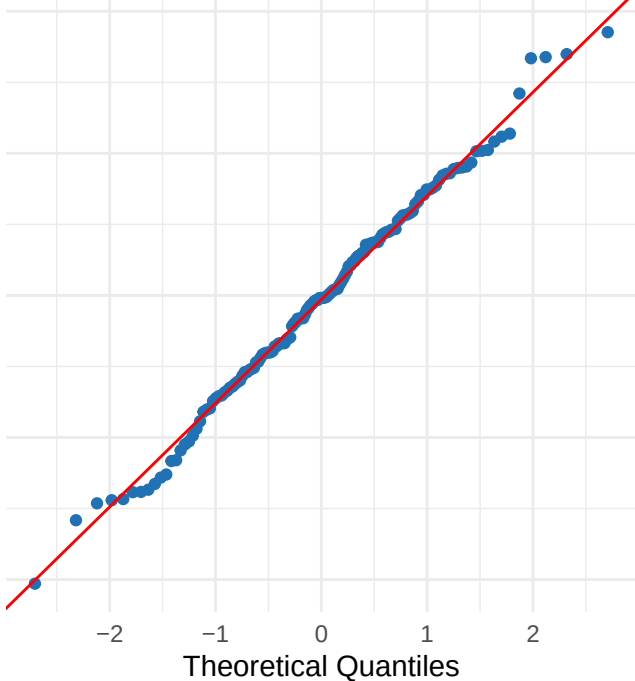
Q-Q Plot of Residuals
