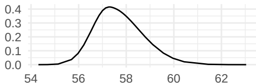
Precision for the Gaussian observations
