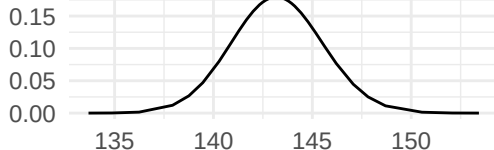
Precision for the Gaussian observations
