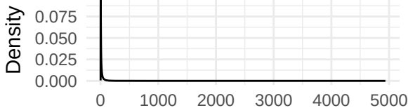
Precision for the Gaussian observations
