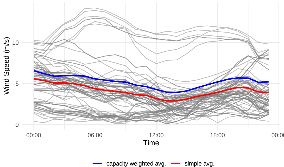
Wind Speed Time Series 2020-08-14
