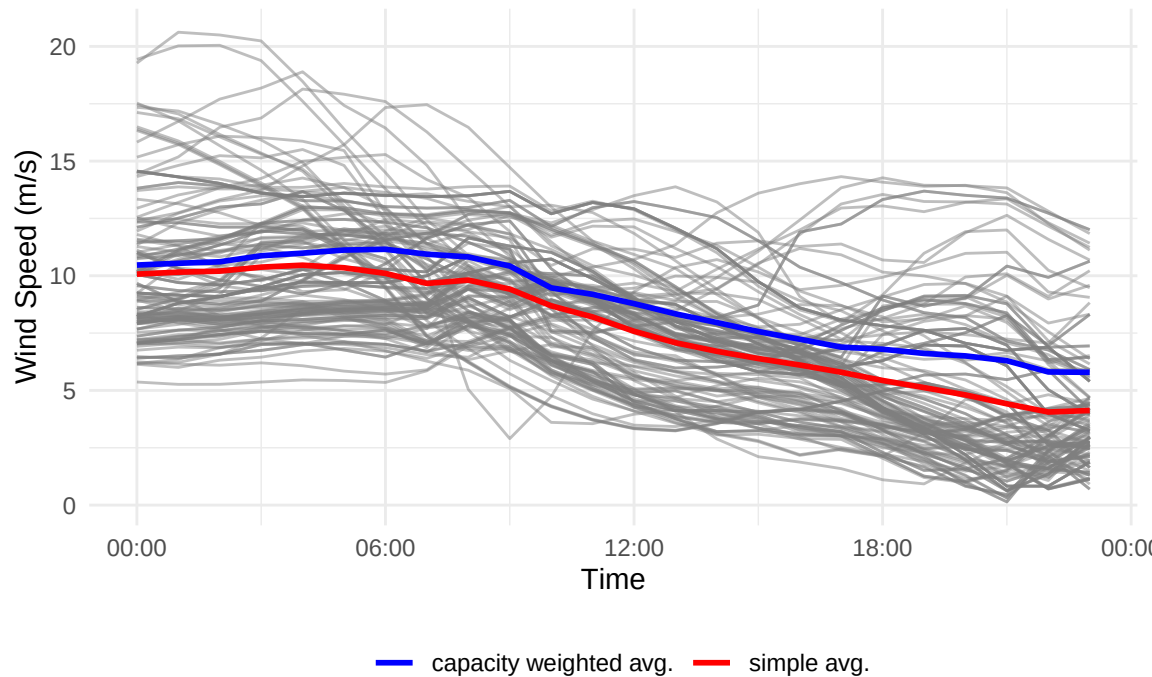
Wind Speed Time Series 2024-04-17
