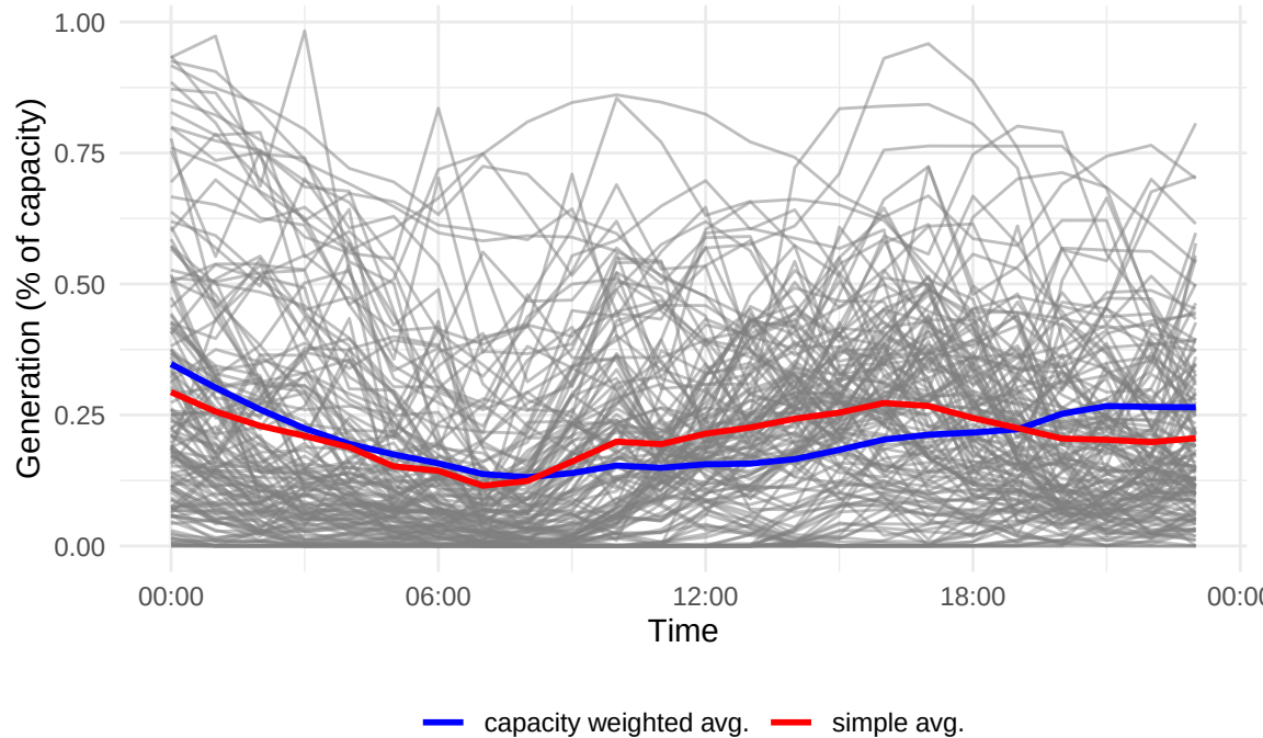
Observed power Time Series 2025-08-10
