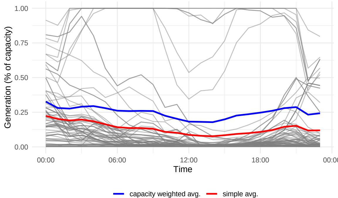
ERA5 + Generic PC Time Series 2020-08-14
