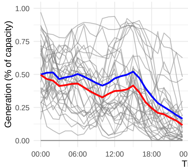
Wind Offshore
