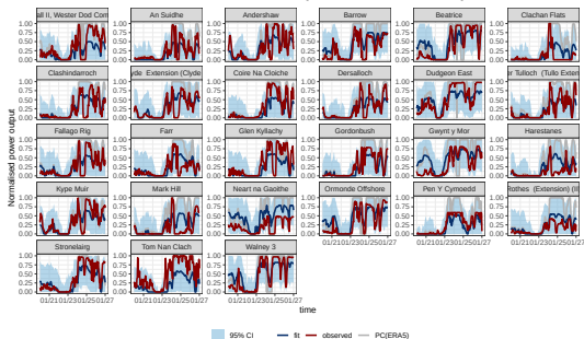
Linear model (27-01-2025)
