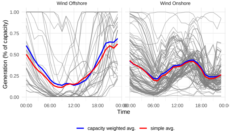
ERA5 + Generic PC Time Series 2025-08-10
