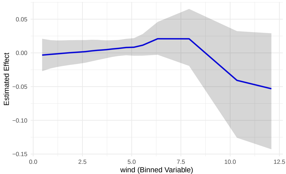
Estimated effect for wind
