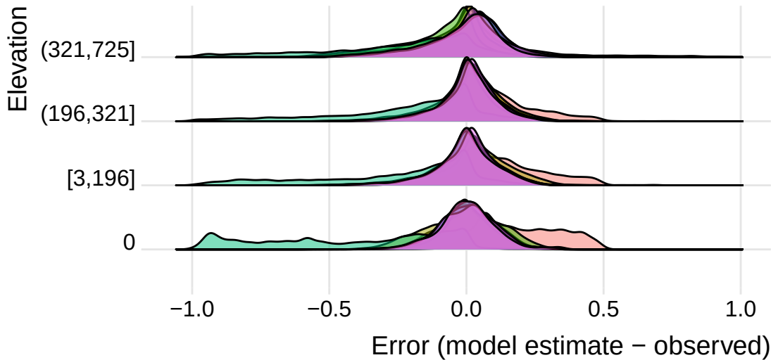
Error distribution by elevation
