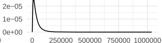
Precision for techno
