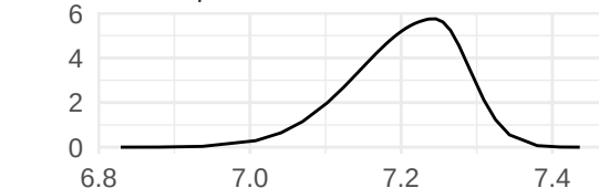
recision parameter for the beta observation
