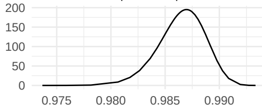
Precision for hour
