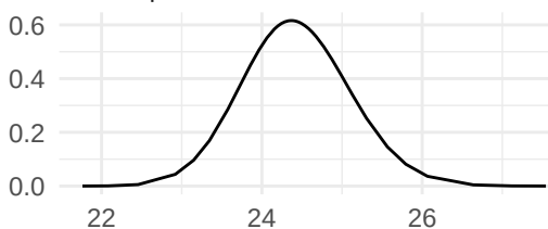
Stdev for spatial
