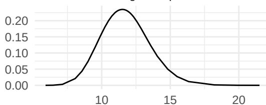
Range for spatial
