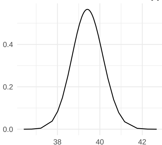
Precision for the Gaussian observations[2]
