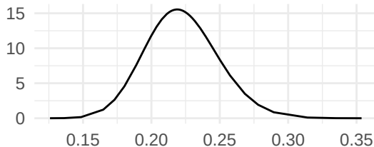
PACF2 for t
