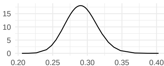
Precision for t
