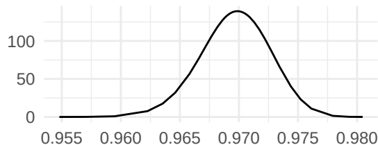
Precision for fcst_group
