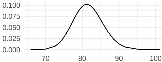
recision parameter for the beta observations[2]
