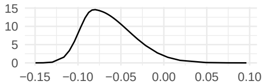
Precision for fd_group
