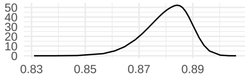
Precision for fcst_group
