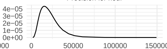
Precision for the Gaussian observations
