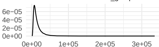
Precision for ws.w_group
