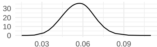
PACF2 for t
