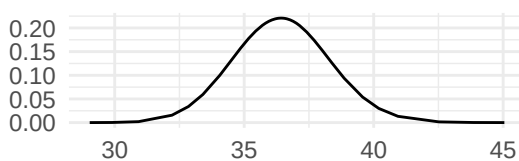
Precision for ws.w_group
