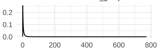
Precision for hour
