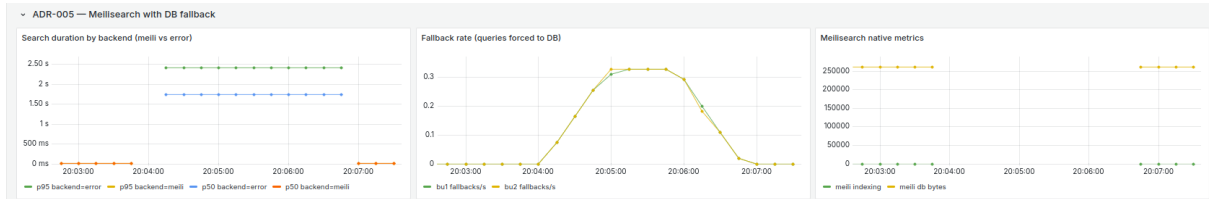
Figure 3: ADR-005 evidence captured during demo-search-fallback.sh . Left: search duration spikes to \sim 2.5 s on the error backend while Meilisearch is paused, compared to \sim 1.6 s on the live path. Center: fallback rate climbs to \sim 0.3 queries/s across both BUs during the outage window, then drops to zero on recovery. Right: Meilisearch native metrics confirm the outage and resumption of the indexing pipeline.
