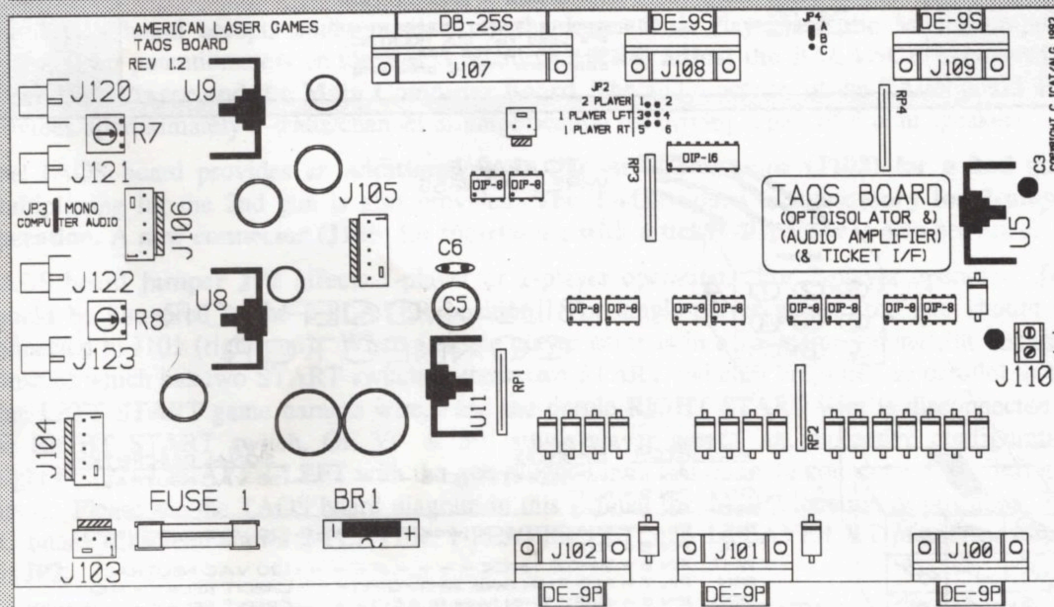
TAOS BOARD (Rev. 1.2) Optoisol/Audio Amplification
