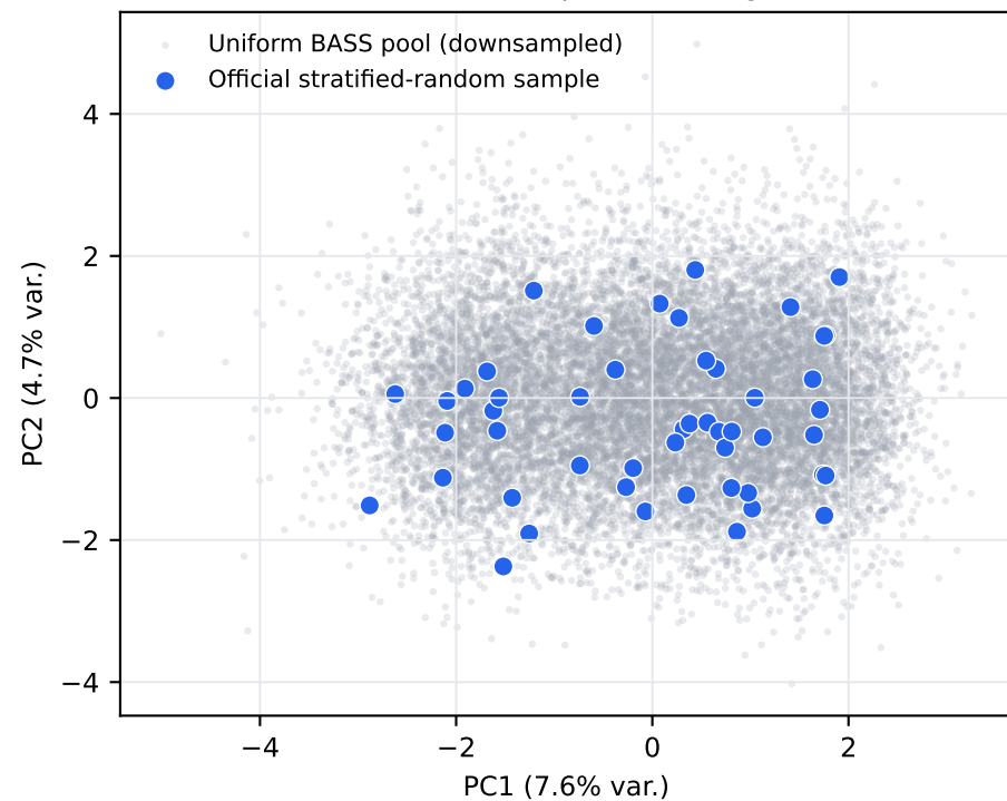
Architecture-space coverage
