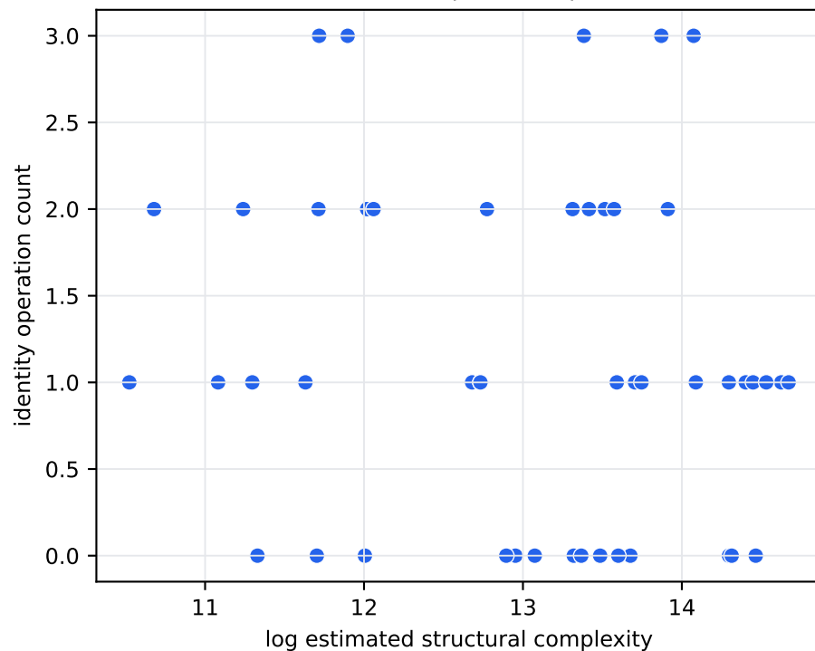
Selected-sample descriptors
