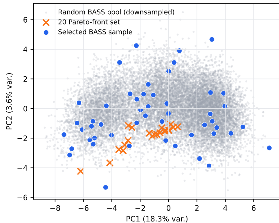
Architecture-space coverage
