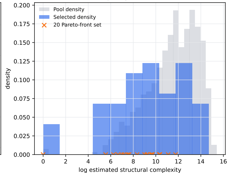
Complexity distribution
