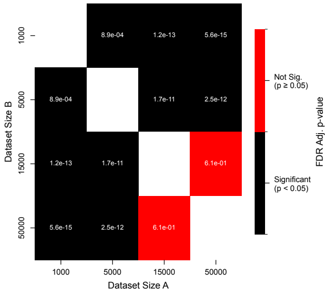
J1: Pairwise Differences (FDR Corrected)
