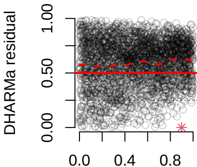
DHARMA residual vs. predicted
