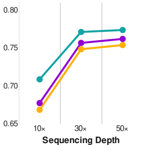
winnow map
