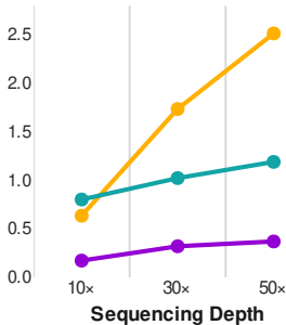
winnomap
