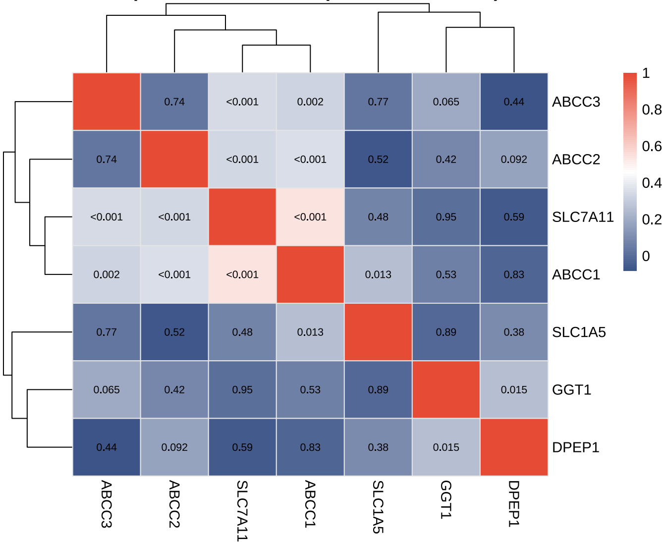
Spearman Correlation (KEAP1-MUT, n=92)
