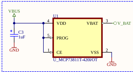
Battery Charger
