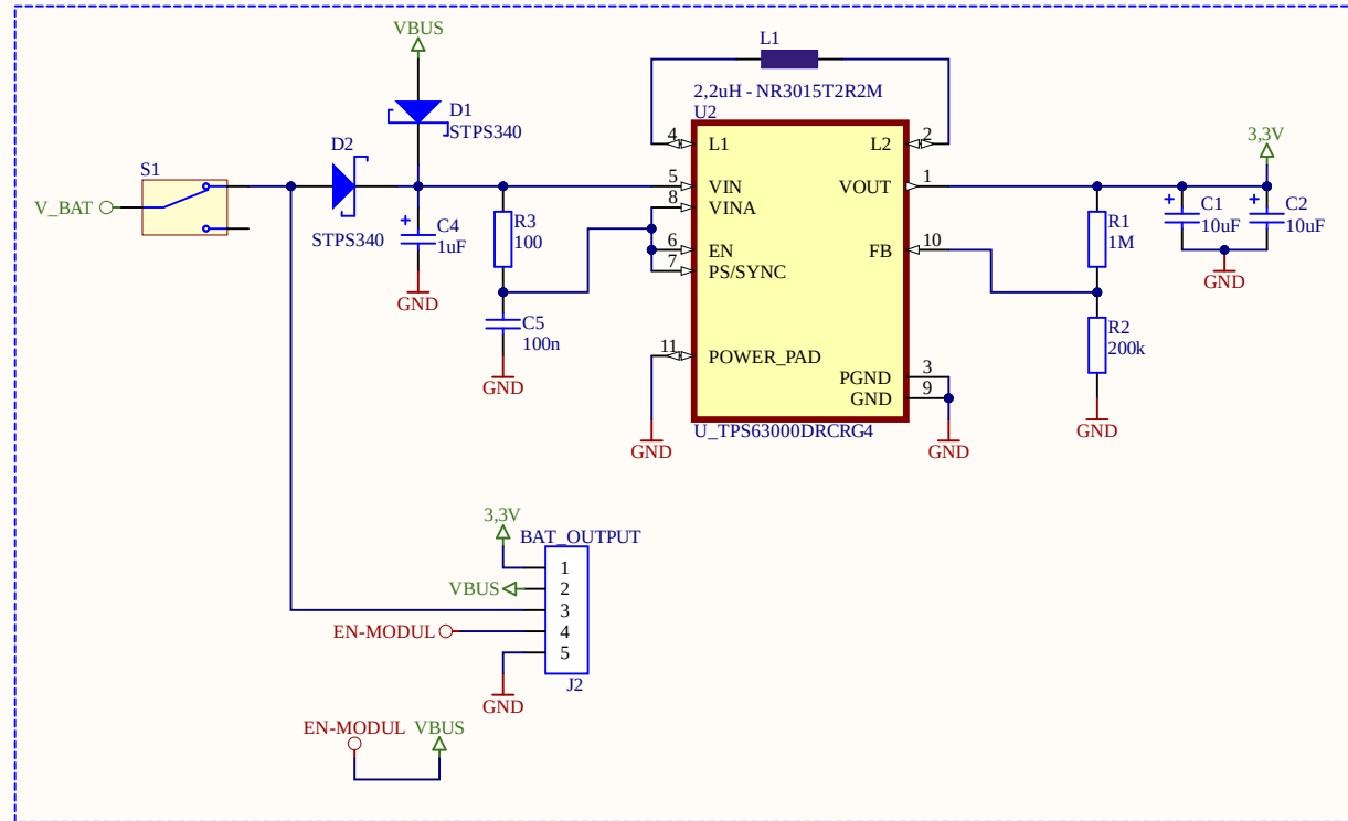
Buck-Boost Converter
