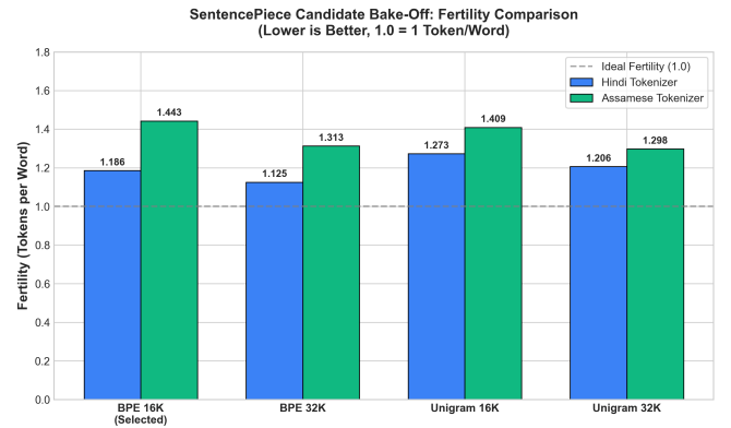
Figure 2: Subword Fertility across Vocabulary Sizes. At 16K vocabulary, Assamese requires 1.4426 tokens/word compared to 1.1858 for Hindi due to Eastern Nagari conjunct ligatures (যুক্তাক্ষৰ).
