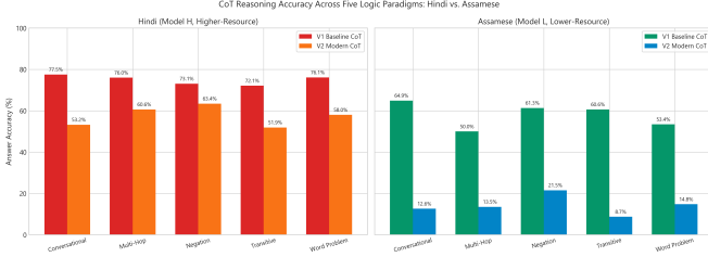
Figure 5: Reasoning Accuracy Across 5 Logic Paradigms. Hindi (left) maintains high cross-paradigm balance ( \sim 72\text{--}77\% ), while Assamese (right) excels in Negation (61.3%) but degrades on multi-hop chains.
