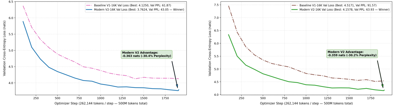
Figure 3: Validation loss over 1,907 steps: Modern V2 vs. Baseline V1. Left Hindi, right Assamese. The legends report best validation loss and perplexity, which are lower than the held-out test figures in Table 3.
