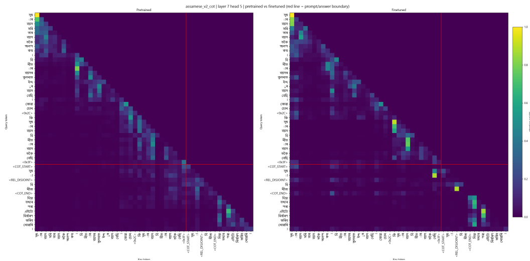
Figure 8: Assamese V2, late layer (layer 7, head 5): pretrained (left) vs. finetuned (right).
