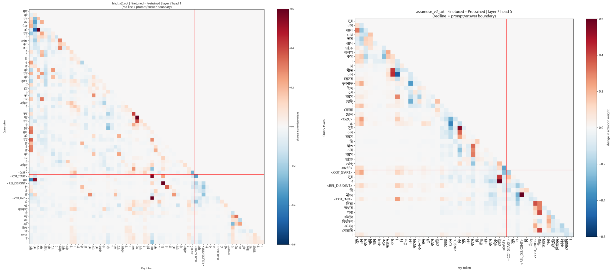
Figure 9: Finetuned minus pretrained attention for the layer-7 heads above (Hindi left, Assamese right). Red = attention gained, blue = attention lost.
