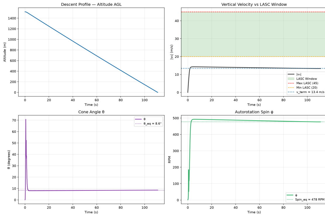
Fig. 3 LRR certification dashboard for the SRAB descent from the real apogee: altitude profile, vertical velocity, cone angle \theta , and autorotation spin rate.
