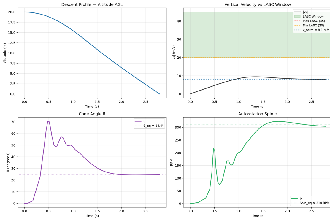
Fig. 8 LRR certification dashboard of Test 2 (Asa2, 4 wings, drone drop from \sim 20 m): the increased wing area ( 122.28 \text{ cm}^2 ) delivers a lower terminal velocity with a stable autorotation state. The alpha-version onboard electronics were validated in this drop, and the data confirmed the need for higher drop altitudes to escape the transient regime.
