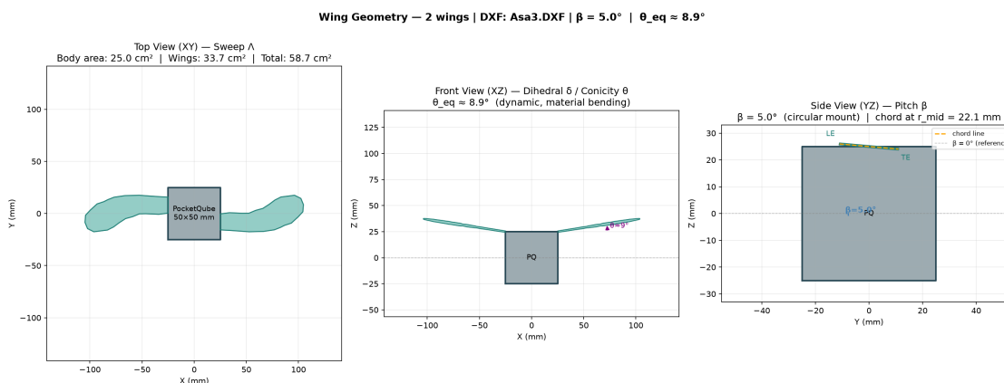
Fig. 2 SRAB wing geometry views: three orthogonal projections of the wing + hub assembly used in the computational simulation and drop tests.
