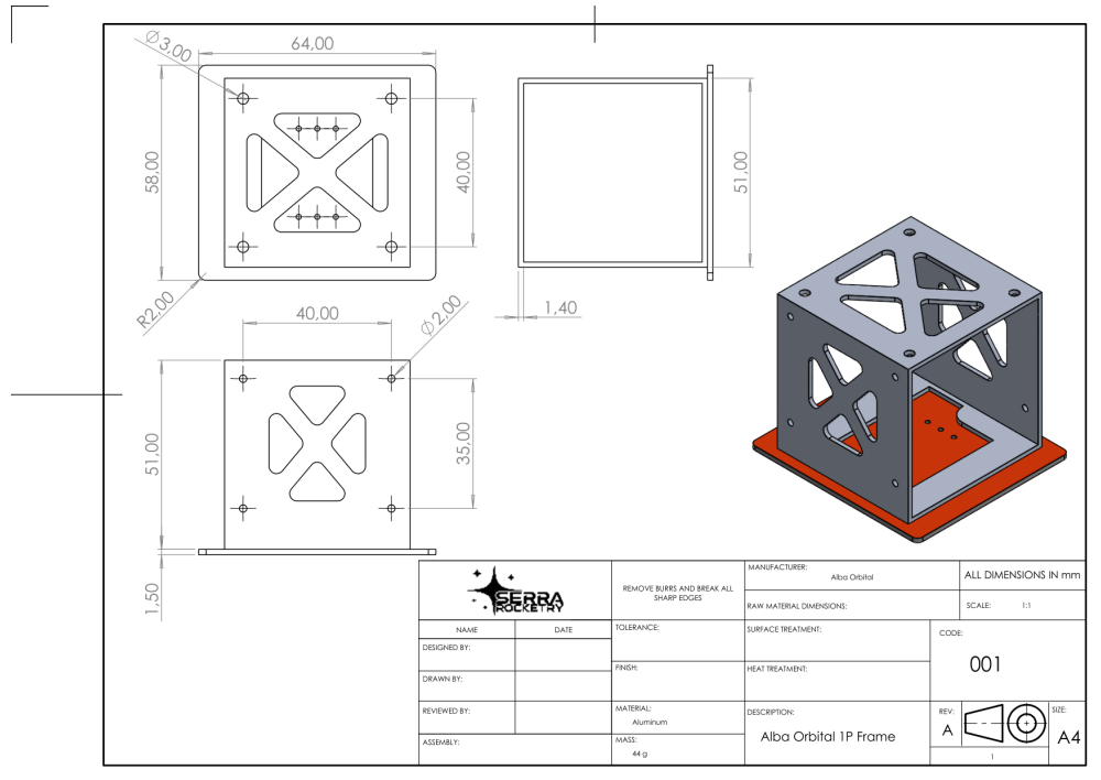
Fig. 10 Technical drawing of the 1P Alba Orbital frame: 51×51 mm aluminum structure with 1.4 mm wall thickness, 1.5 mm FRP backplate and a total mass of 44 g.
