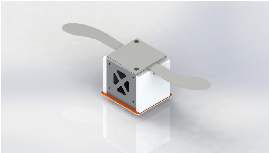
Fig. 1 Complete Helike #213 assembly render: 1P Alba Orbital aluminum frame, FRP backplate and the two SRAB autorotative wings in the deployed configuration.
