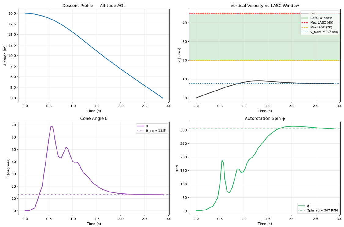
Fig. 7 LRR certification dashboard of Test 1 (Asa1, 4 wings, drone drop from \sim 20 m): altitude profile, vertical velocity against the LASC window, cone angle and autorotation spin rate, converging to the equilibrium values.
