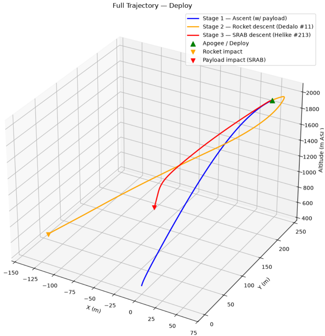
Fig. 5 Full simulated flight of the Dédalo launch vehicle carrying the Helike payload: Stage 1 ascent with payload (blue), Stage 2 rocket descent (orange) and Stage 3 SRAB descent (red), with the deployment event at apogee and the two separate impact points.
