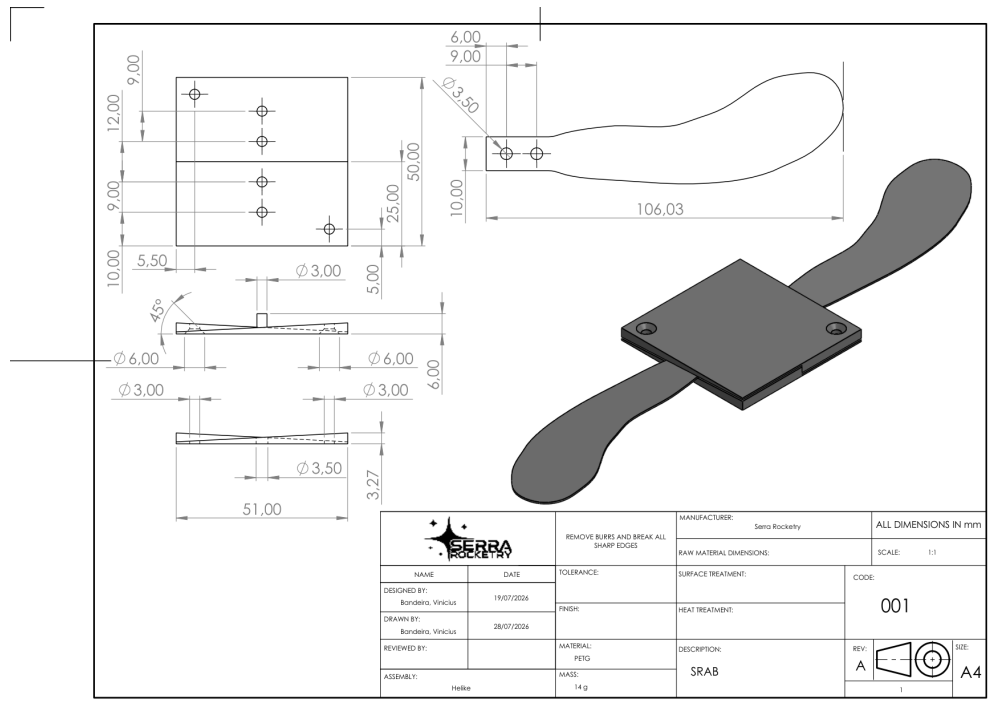
Fig. 11 Technical drawing of the SRAB assembly: central 50×50 mm hub and the two mirrored autorotative wings (PETG, total mass 14 g).
