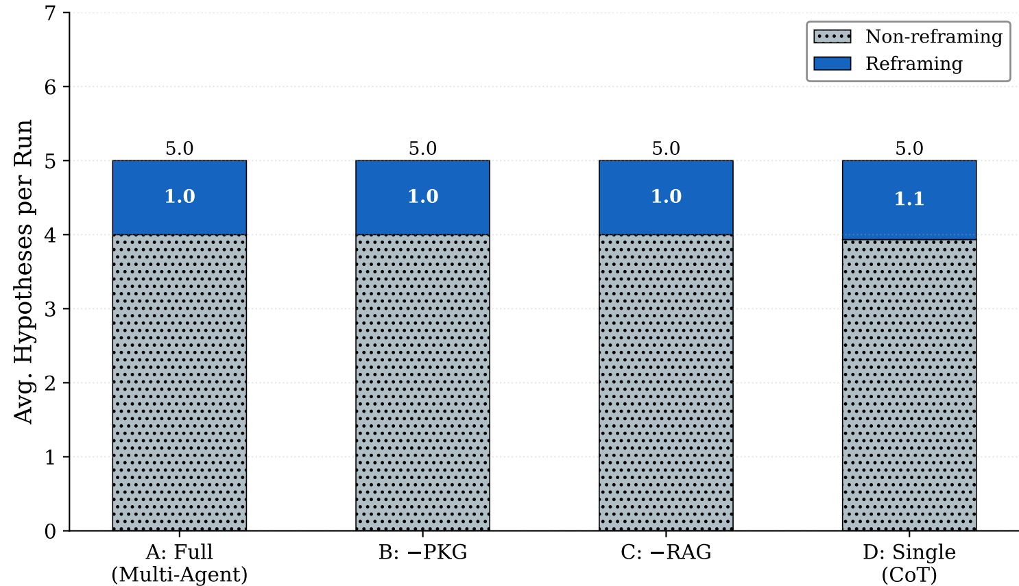
Hypothesis Composition by Condition
