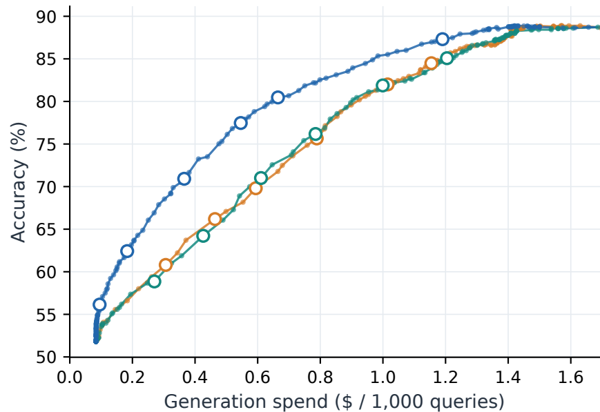
LiveCodeBench · 341 original test problems
