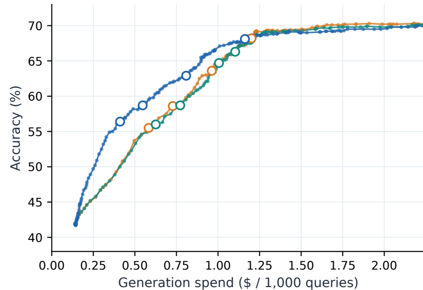
Omni-MATH · 1,000 new problems
