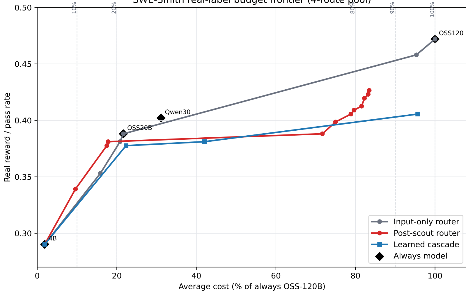
SWE-Smith real-label budget frontier (4-route pool)
