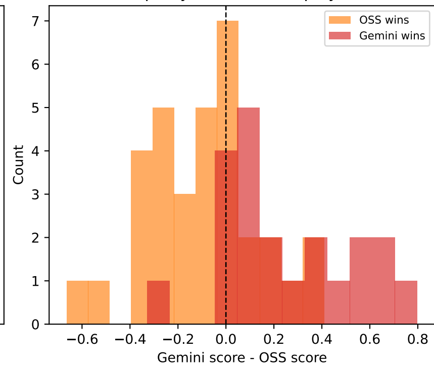
True proxy delta (non-deployable)
