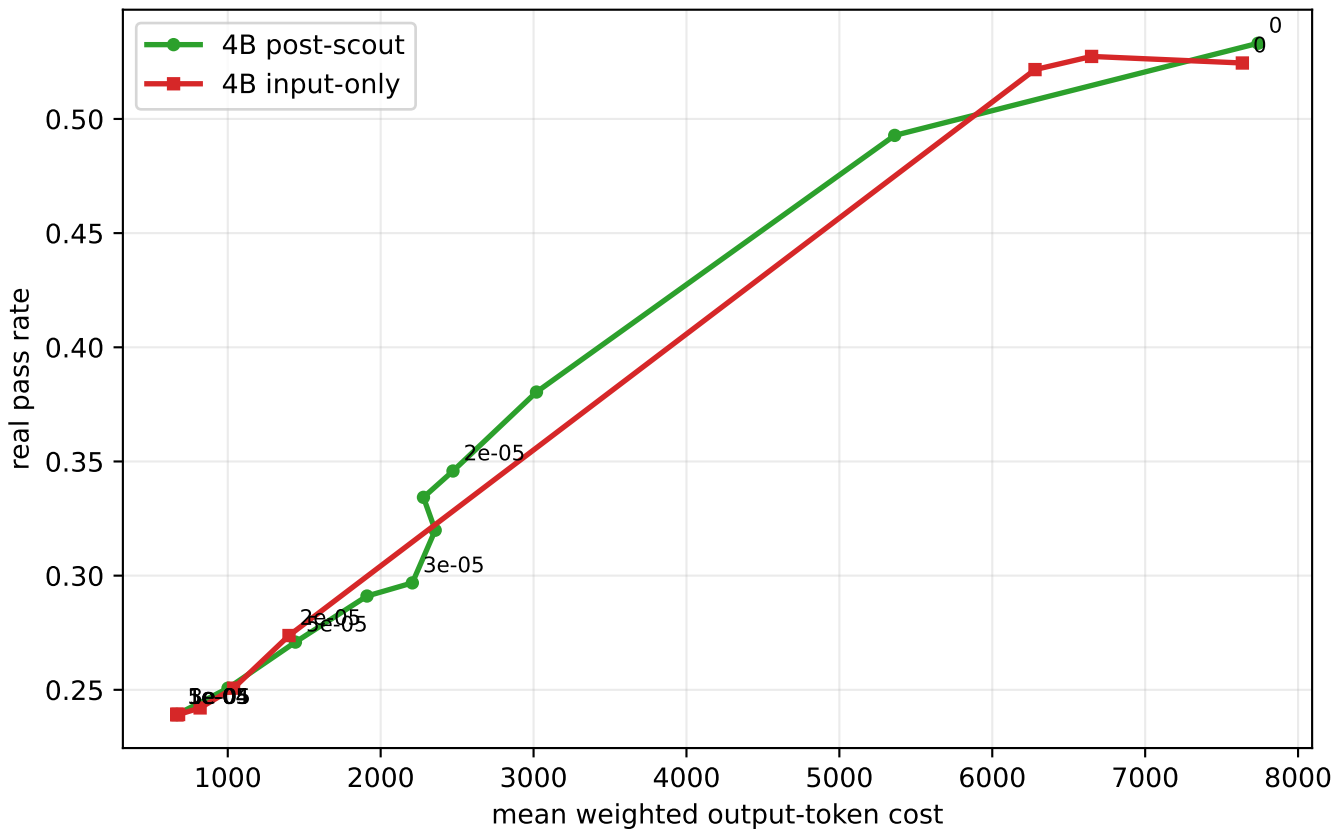
4B scout real reward-cost tradeoff
