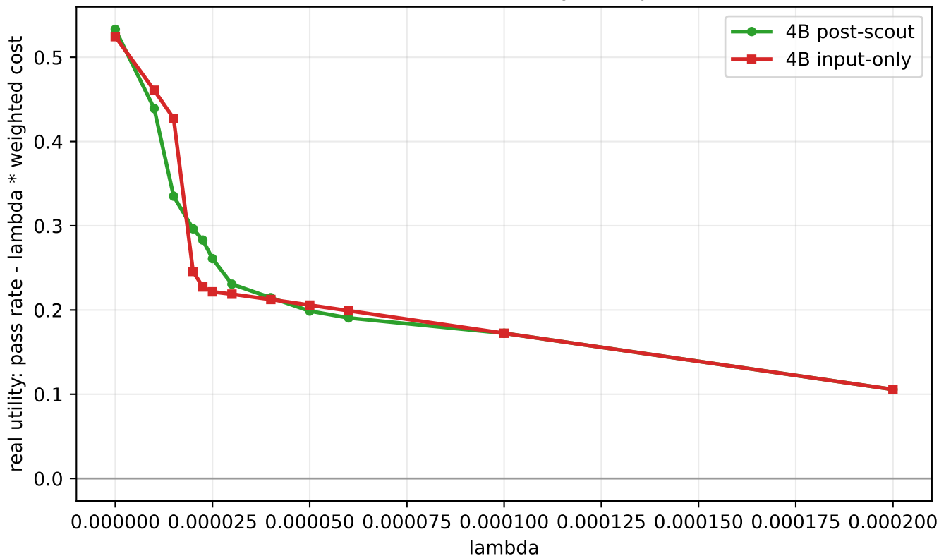
4B scout real utility sweep
