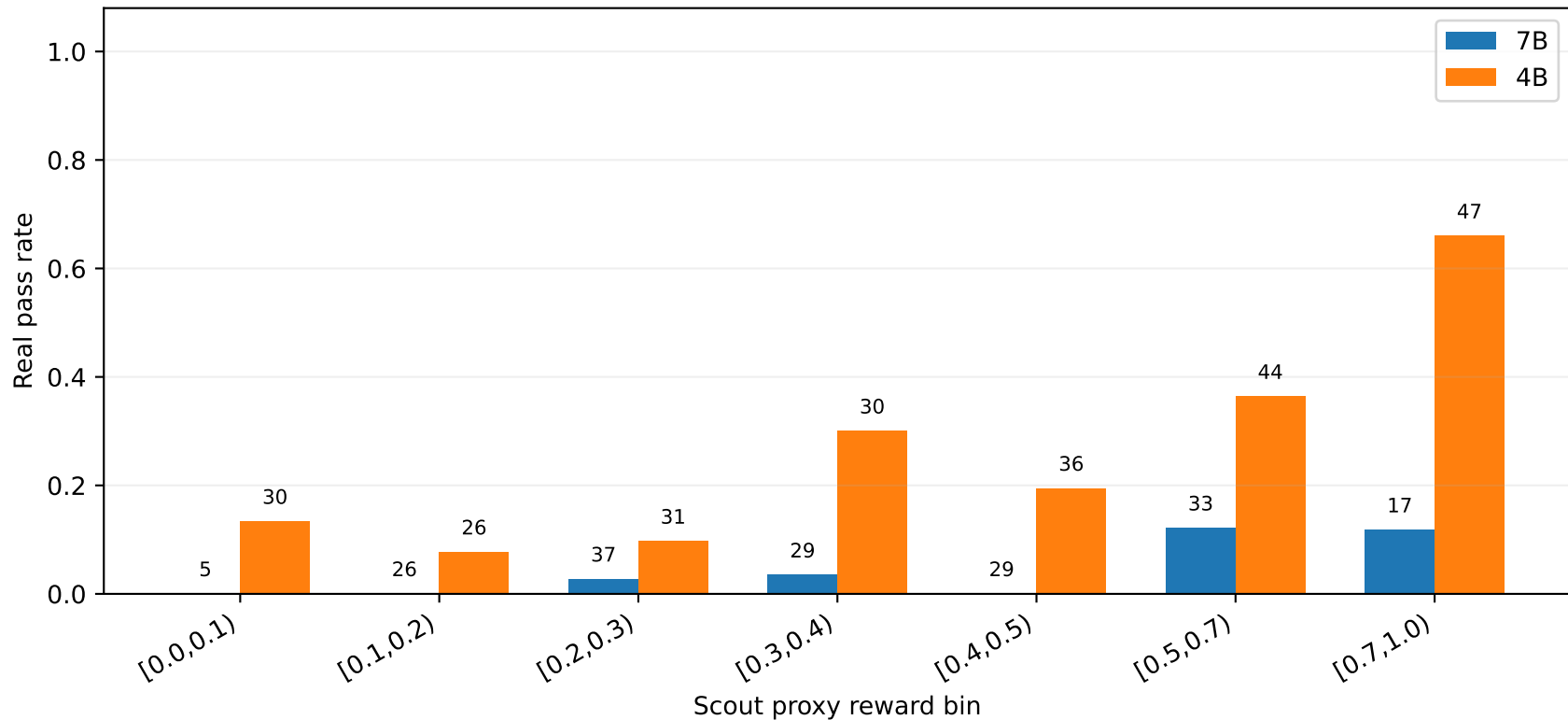
Scout-selected real pass rate by proxy bin, \lambda=2e-05
