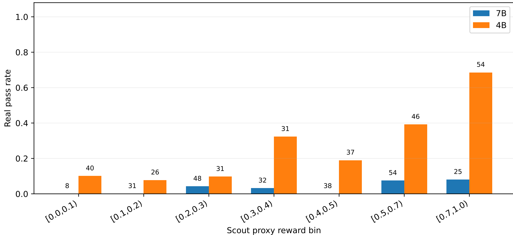
Scout-selected real pass rate by proxy bin, \lambda=3e-05
