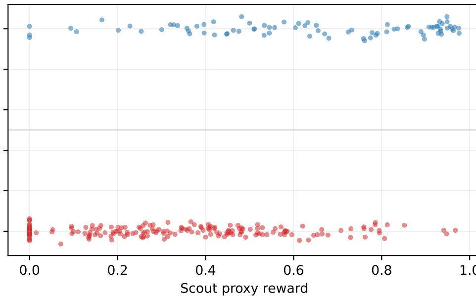
4B lambda=3e-05: n=265, pass=30.6%
