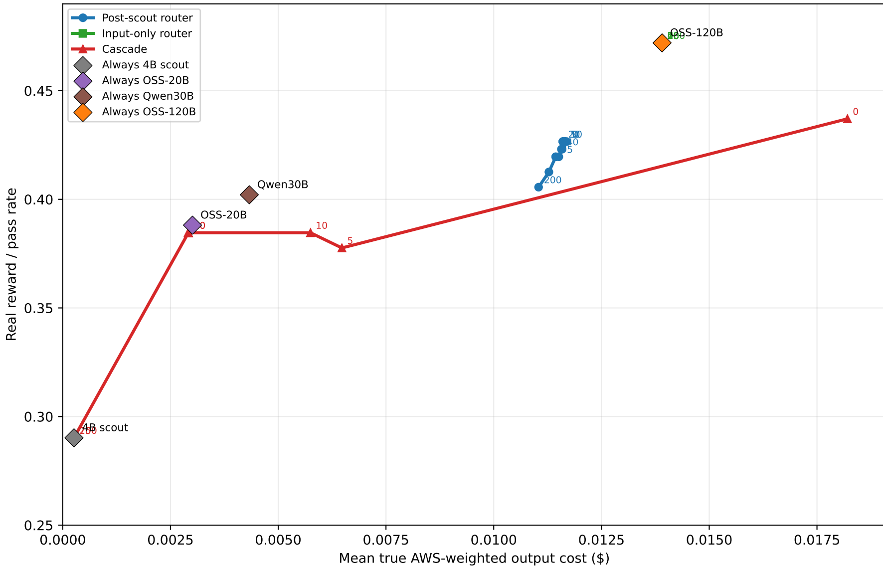
Real Reward vs. Cost on SWE-Smith Eval (286 examples)
