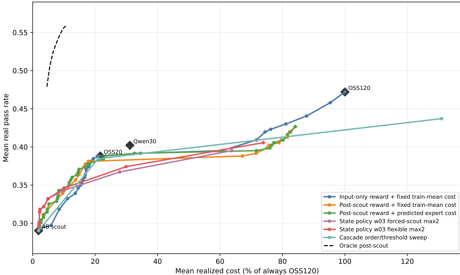
SWE-Smith real reward vs realized AWS-weighted cost
