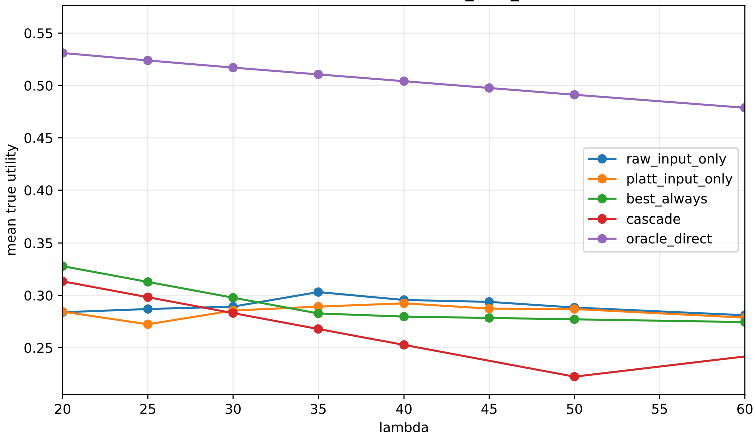
Bare direct calibration (fixed_train_mean)
