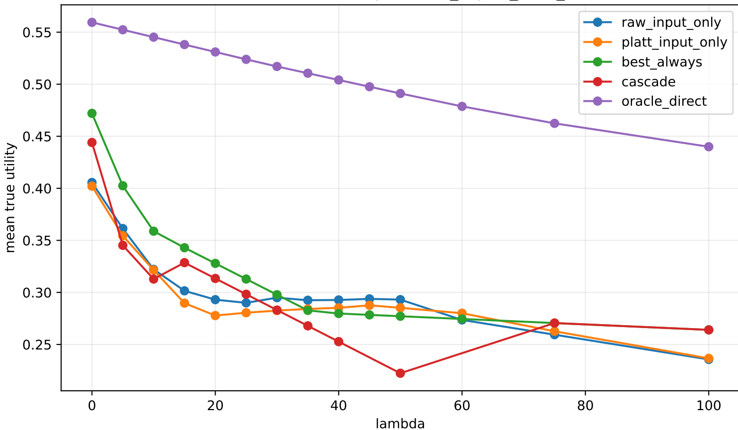
Bare direct calibration (predicted_expert_fixed_scout)
