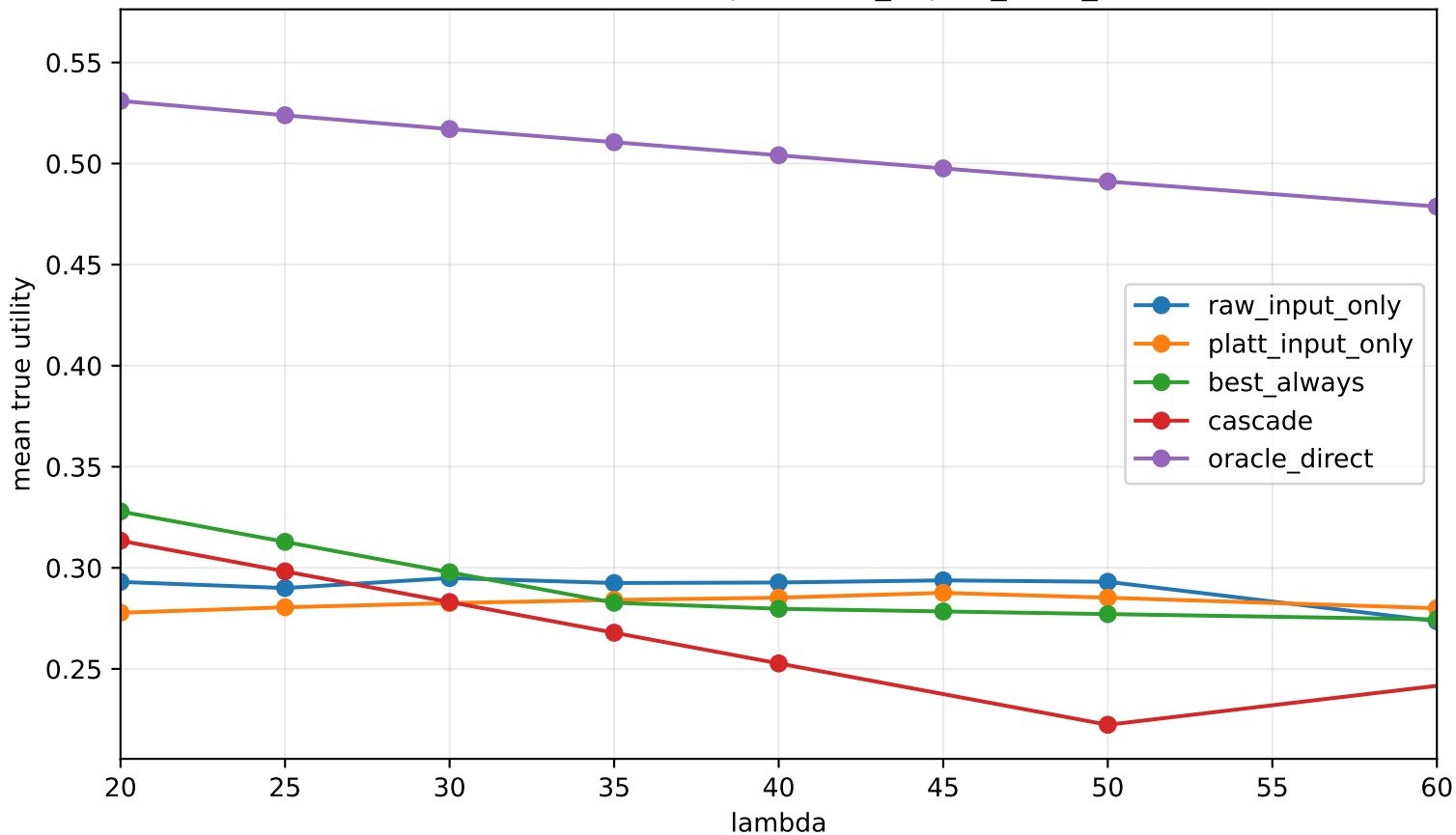
Bare direct calibration (predicted_expert_fixed_scout)
