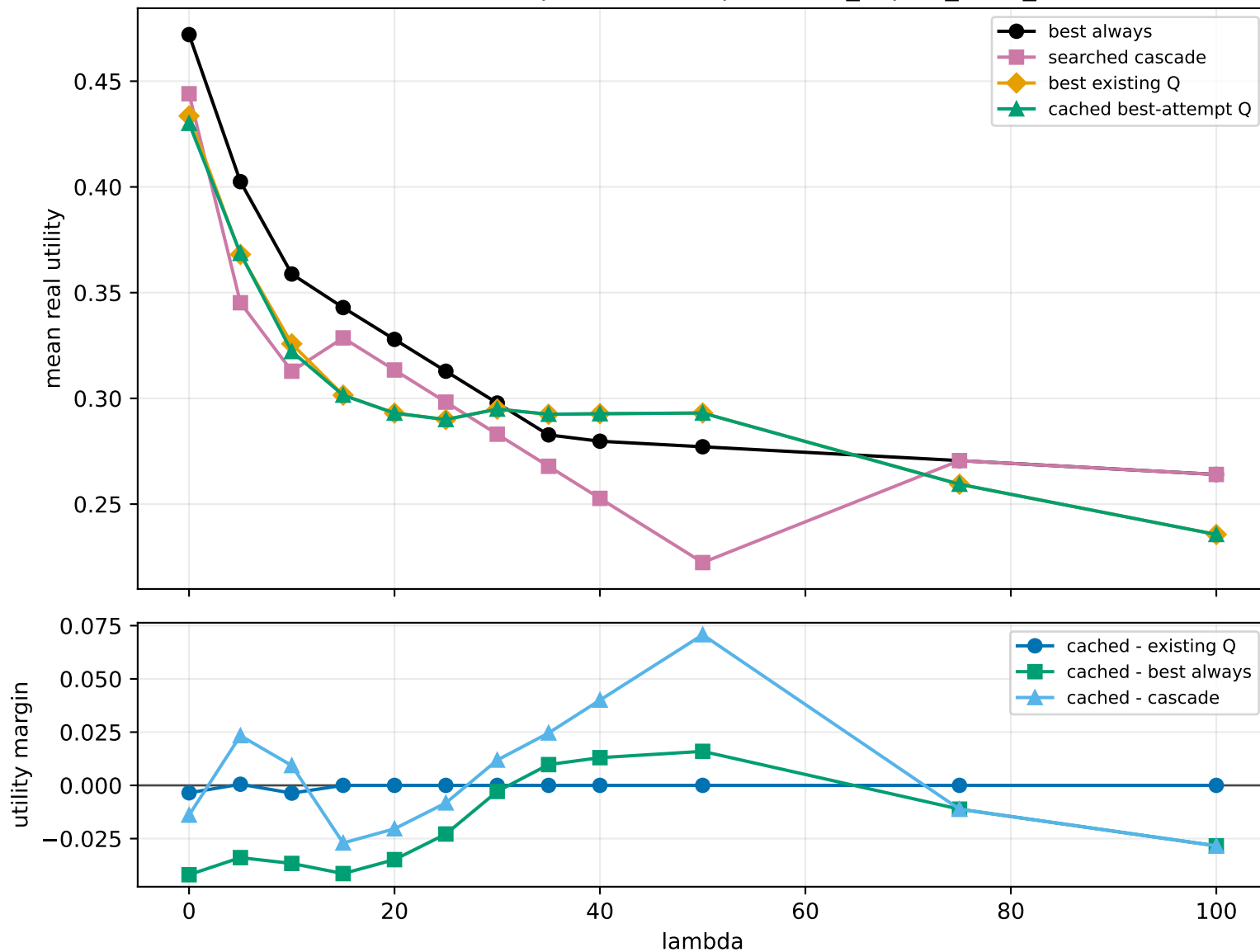
Cached best-attempt Q rescore (predicted_expert_fixed_scout)
